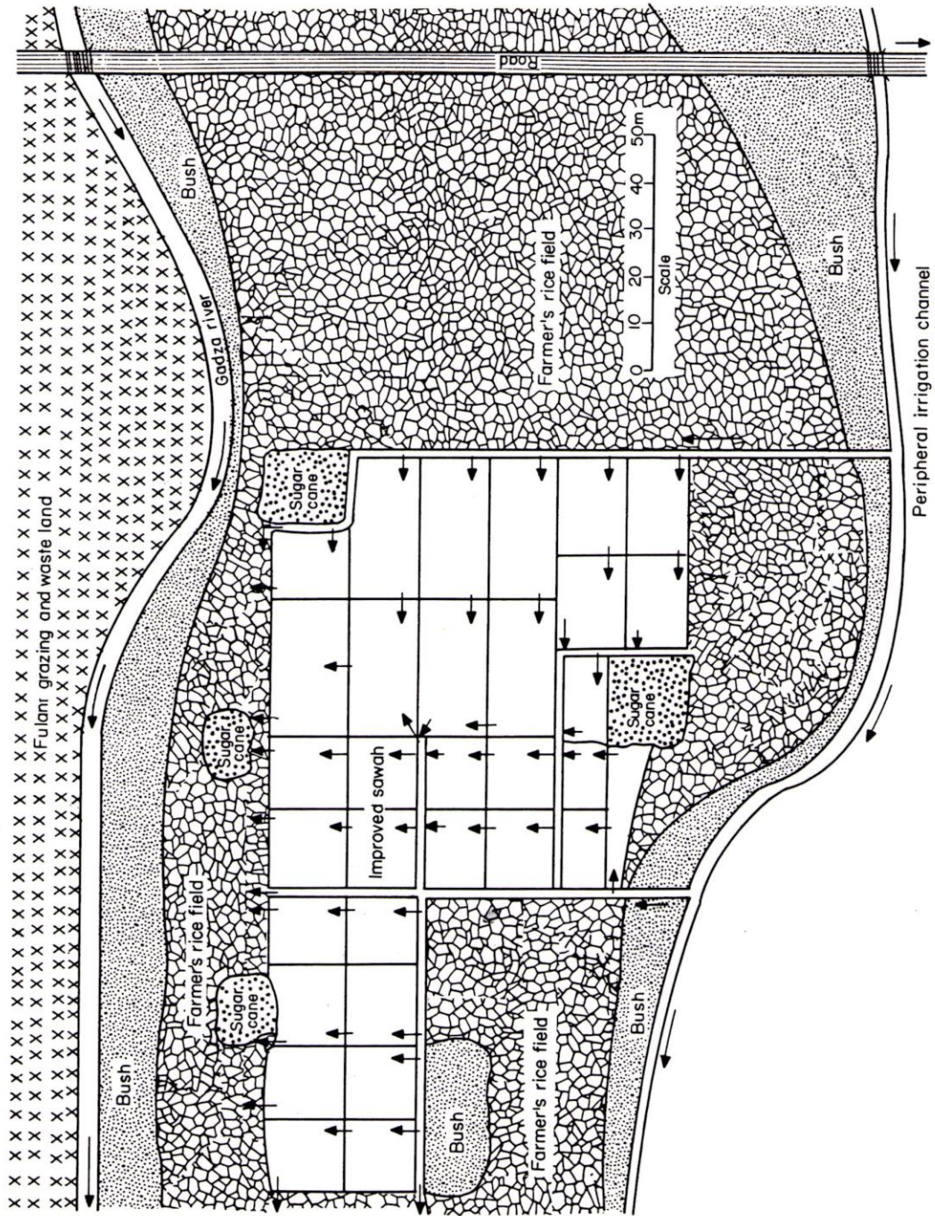
Figure 7.5. Sketch of farmers' rice fields and improved paddy (sawah) at Gadza, Bida, Nigeria, November, 1987
