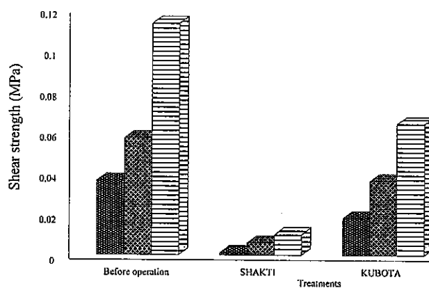
Fig. 2. Shear strength before and after tillage operations for the investigated depths: 0-7, 7-14, and 14-21 cm from left to right.
