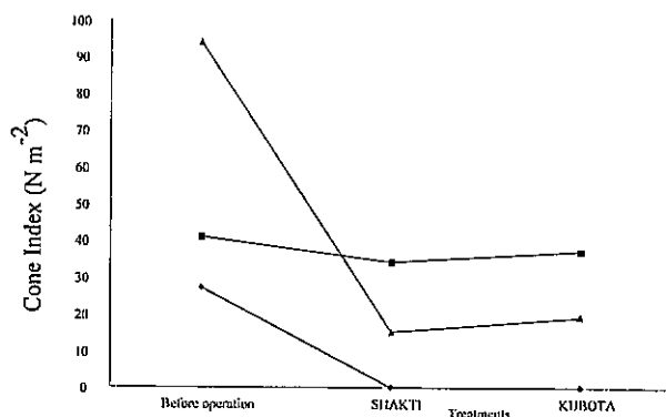
Fig. 3. Cone index before and after tillage operations. ◆ 0-7 cm, ■ 7-14 cm, ▲ 14-21 cm.
