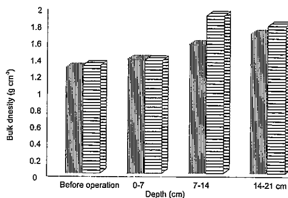
Fig. 1. Bulk density before and after tillage operations., SHAKTI – left, KUBOTA – right.
